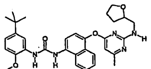
1-(5-tert-Butyl-2-methoxy-phenyl)-3-(4-{6-methyl-2-[(tetrahydrofuran-2-ylmethyl)amino]-pyrimidin-4-yloxy}-naphthalen-1-yl)-urea;
